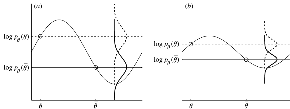
Figure 5. The discrimination parameter \sigma is undetermined. (a) Graph of an example log prior, \log p_\theta(\theta) (solid horizontal sinusoid curve), as a function of lighting direction \theta . Given two hypothetical neurons with preferred lighting directions \theta and \bar{\theta} , their responses are determined by their log probability density functions, \log p(\theta) and \log p(\bar{\theta}) , indicated by the vertical dashed and solid curves, respectively. For a given stimulus, the larger of the two observed values from the probability density functions \log p(\theta) and \log p(\bar{\theta}) determines the lighting direction assumed by the observer, and this, in turn, determines the concave/convex observer response. These two observed values are noisy estimates of the probability density function means, so the choice probability q (see equation (2.19)) is determined by the relative overlap of the probability density functions (vertical dashed and solid curves) for these two quantities. (b) A log prior with amplitude variations k times smaller than in (a) leads to the same choice probabilities as in (a), provided the noise level \sigma is also reduced by a factor k . (For simplicity, this analysis assumes a concavity preference of 0.5.)
